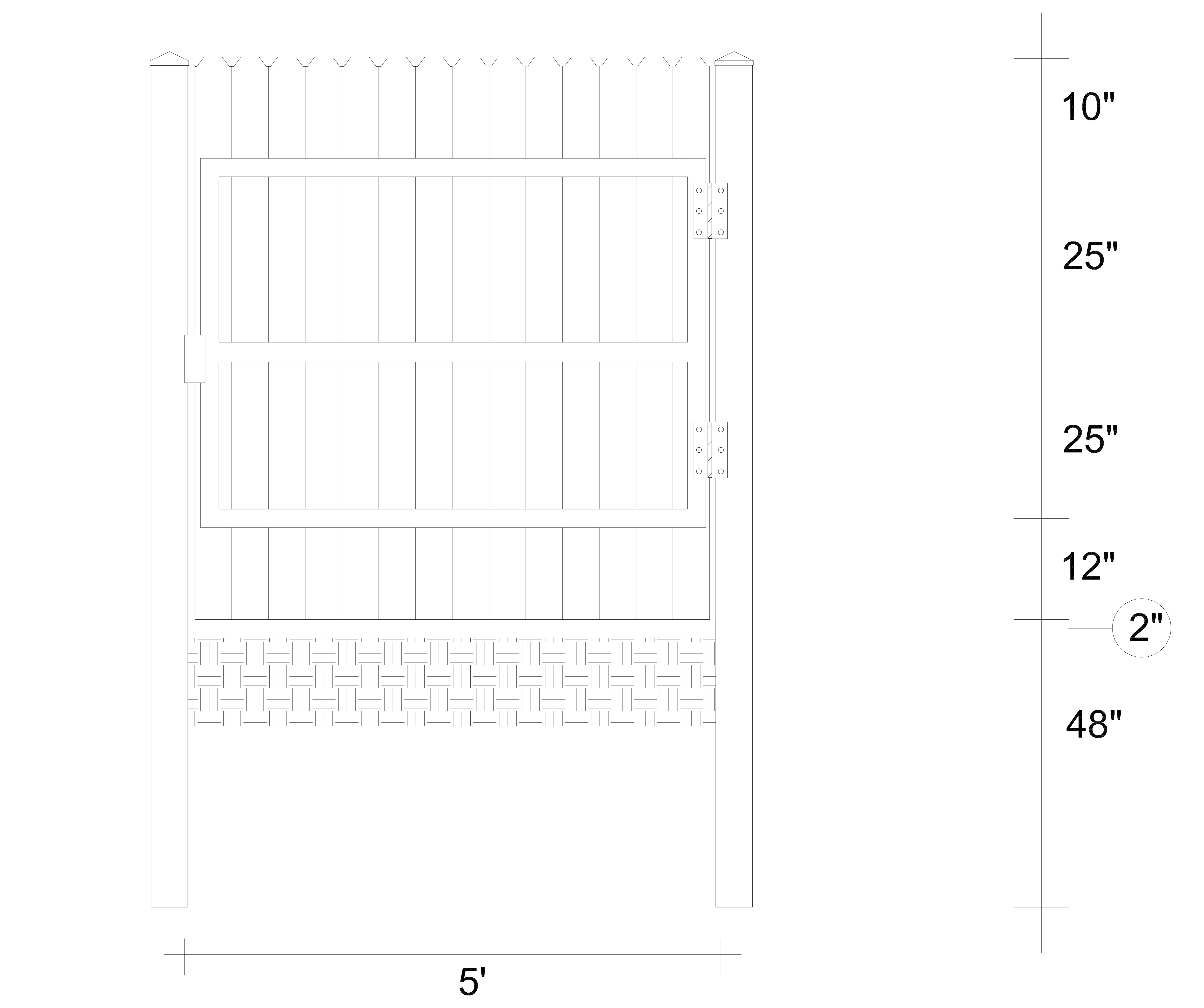
SINGLE GATE 6' X 5' REAR VIEW
