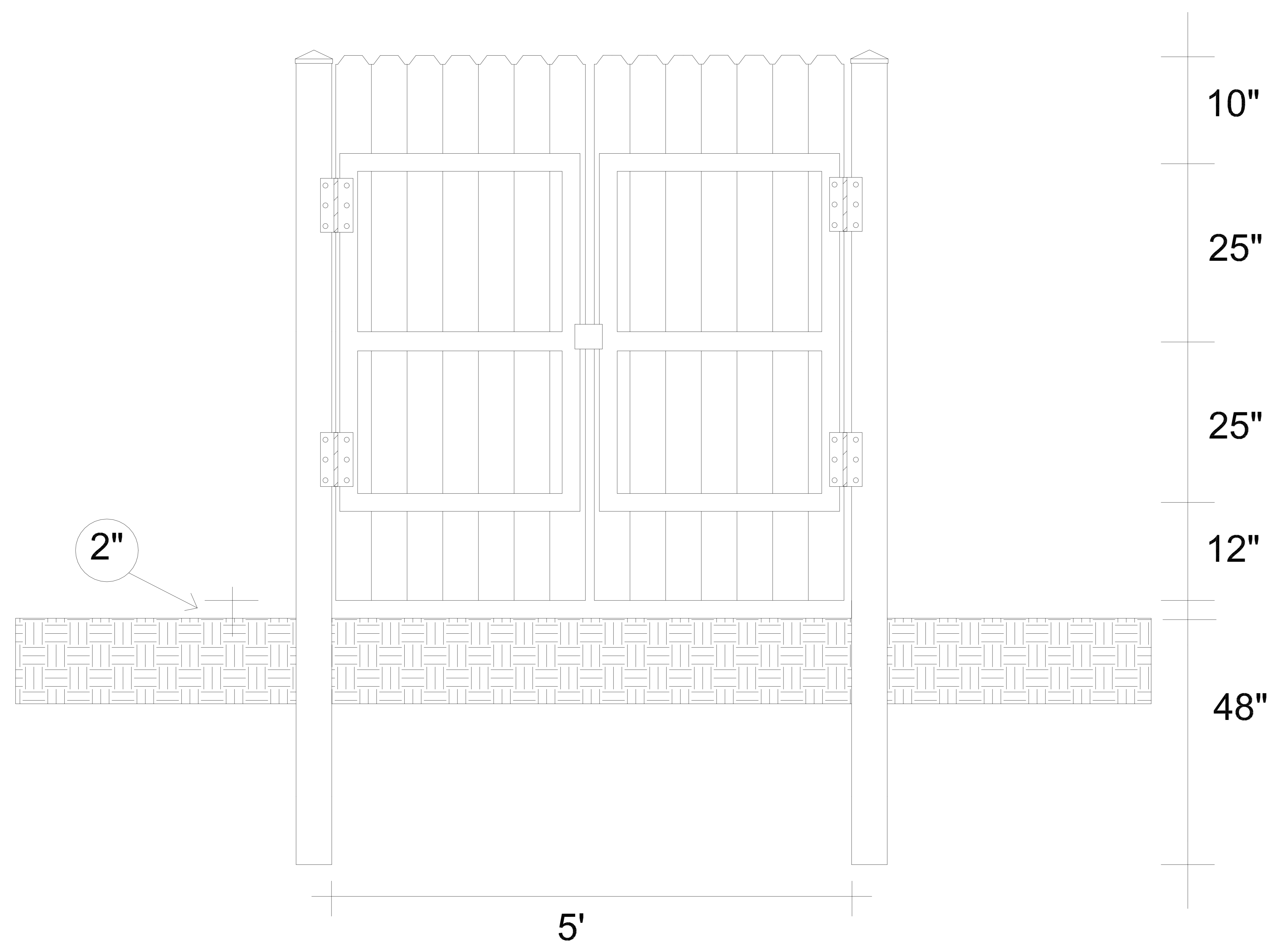
DOUBLE GATE 6' X 5' REAR VIEW
